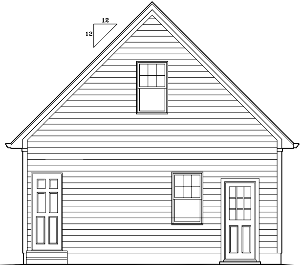
Side Elevation
